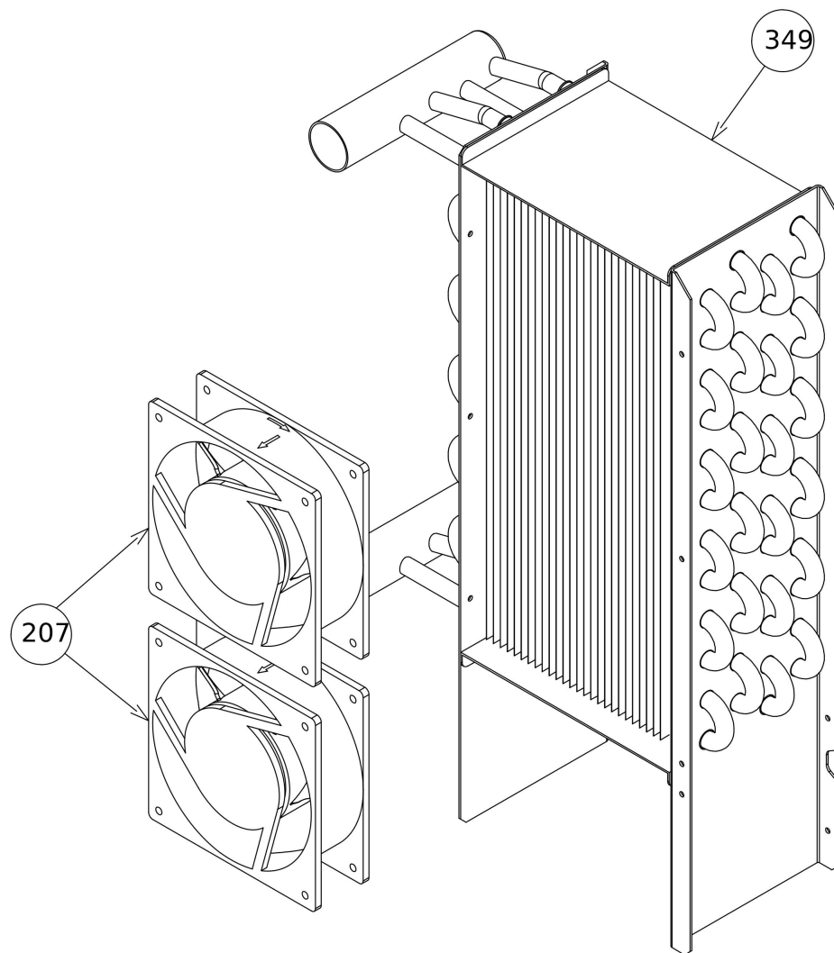
Condensing unit
